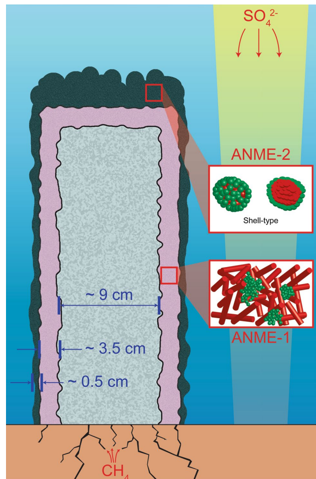
Fig. 1 Representation of the microbial reefs found in the Black Sea. Microbial reef structures form over methane seeps in the SMTZ. The inner structure is a porous carbonate precipitate (grey) [90]. The carbonate is covered by a layer of ANME-1 (pink) in a mat-type consortium. The outer layer (black) is composed of ANME-2 in shell-type consortia. This layer is described as nodular and is thicker at the top of the reef. In the insets, the ANME cells (red) and SRB cells (green) have colors matching those visualized by FISH [41]. The sizes of microbial reefs vary but estimates were provided by Treude et al. [91]. Descriptions of color and photos of the structures can be found in several works [41, 43, 73] (color figure online)
