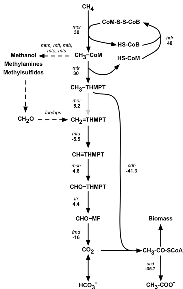
Fig. 2 Reverse methanogenesis pathway. The Mer enzyme (grey) is found in ANME-2 but not ANME-1. The proposed alternative pathway for ANME-1 by Meyerdieckers et al. [53] is shown in dotted arrows. Gene names are italicized and \Delta G values (in bold below gene names) are from Thauer [86] with updated values for Mcr [81] and Fmd [87] (color figure online)
